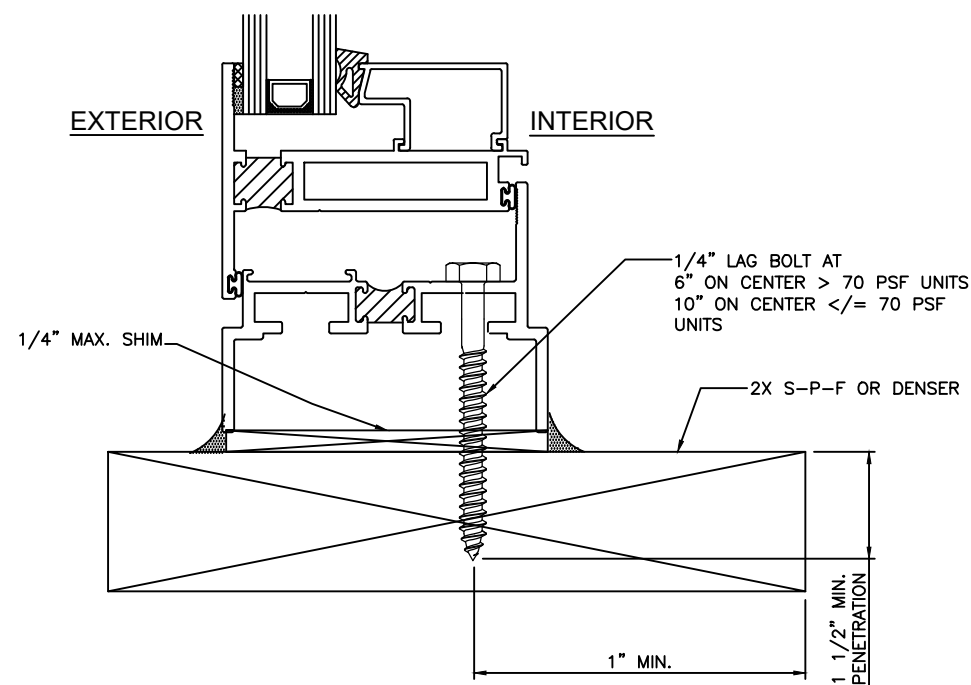
SECTION 1/1, 1/2 & 1/3 THROUGH FRAME TO WOOD FRAMING OR BUCK
